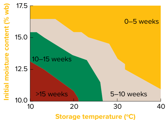
Figure 1: Estimated safe storage life of rye based on 20% decrease in the initial germination and no visible mould. Periods of safe storage are indicated. 8
