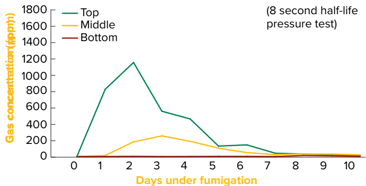
Figure 3: Gas concentration in non-gas-tight silo.
